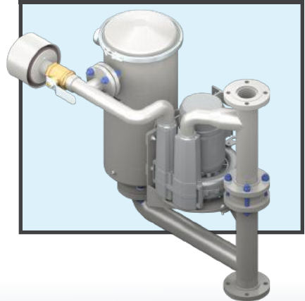
Bypass Option
